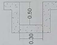
Drain cross section
